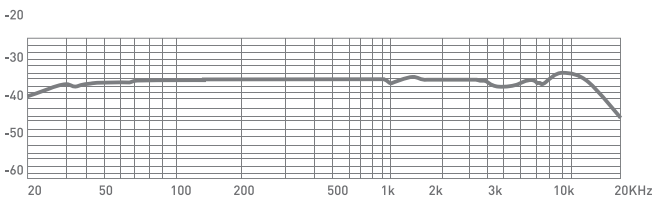
Frequency Response Curve
